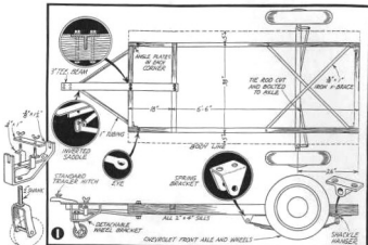
1 6" WHEEL
